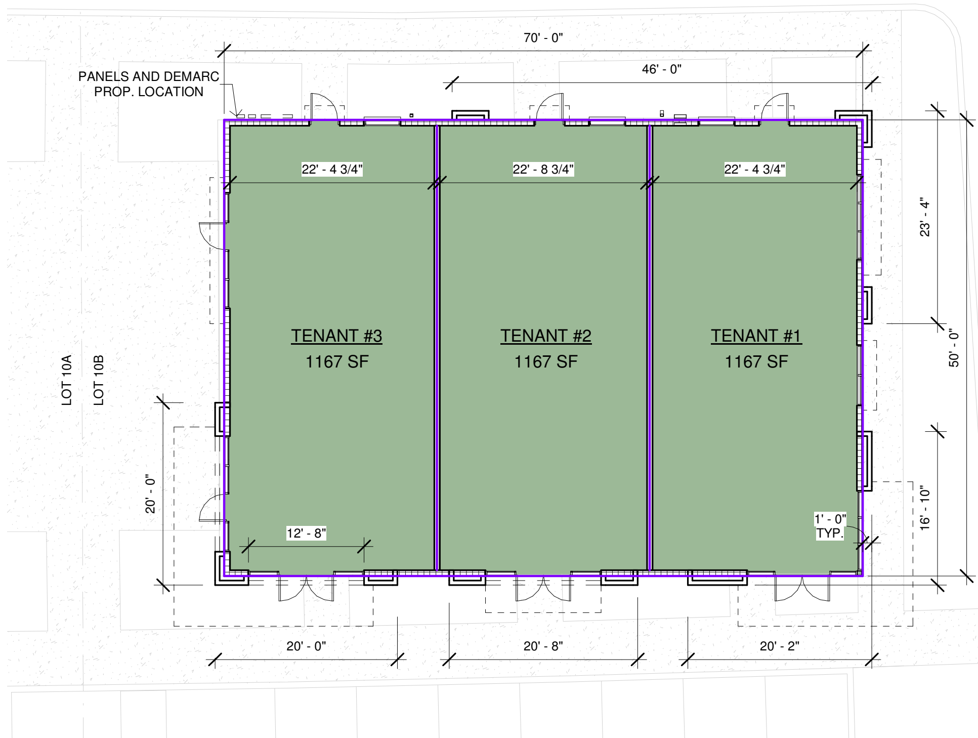
FLOOR PLAN 3,500 SF TOTAL
