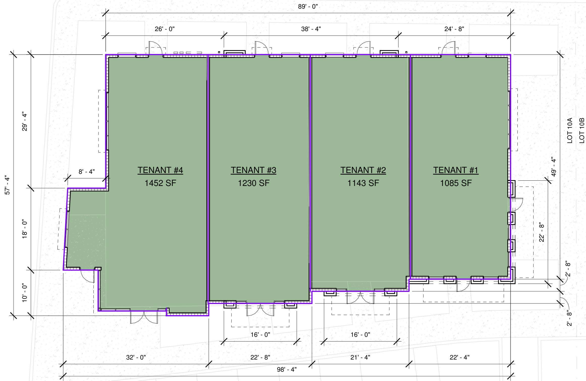
FLOOR PLAN 4,910 SF TOTAL
